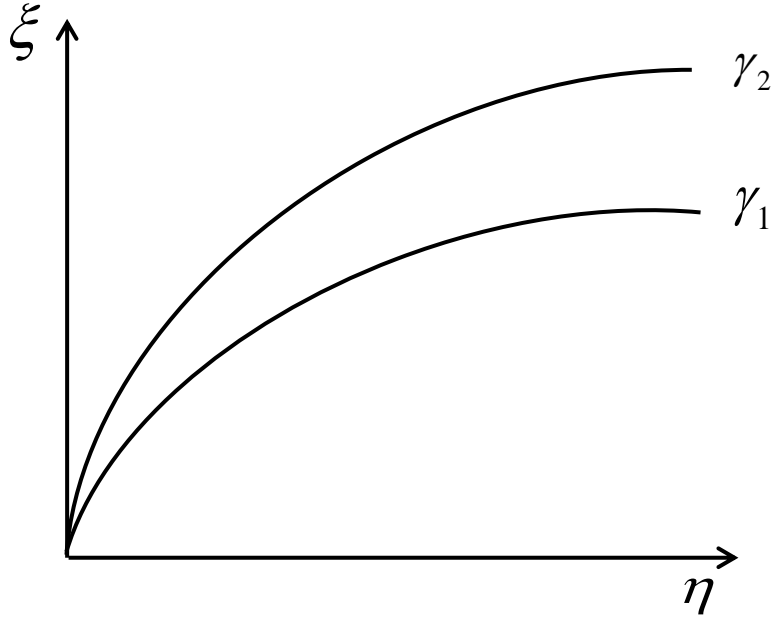
Figure 4: Effects of Stocking Rate on Soil Organic Matter and Energy Production.
