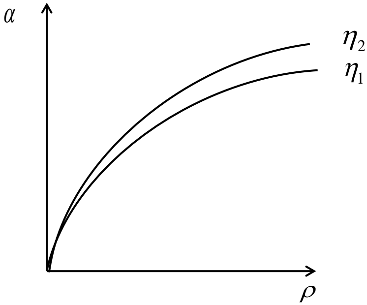
Figure 2: Effects of Soil Organic Matter on Pasture Mass and Beef Production.
