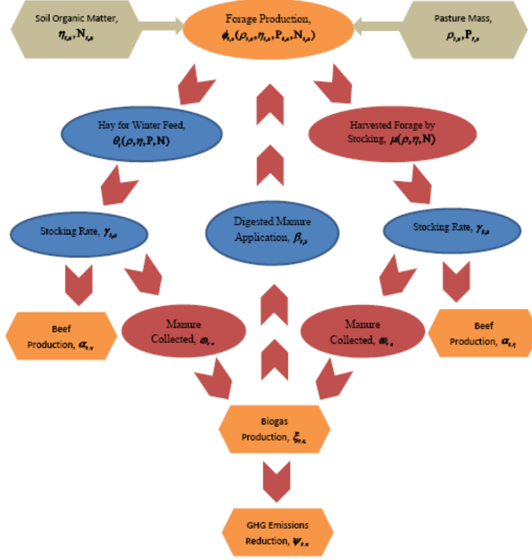
Figure 1: Paths of Soil Organic Matter and Pasture Mass in Locations z .
