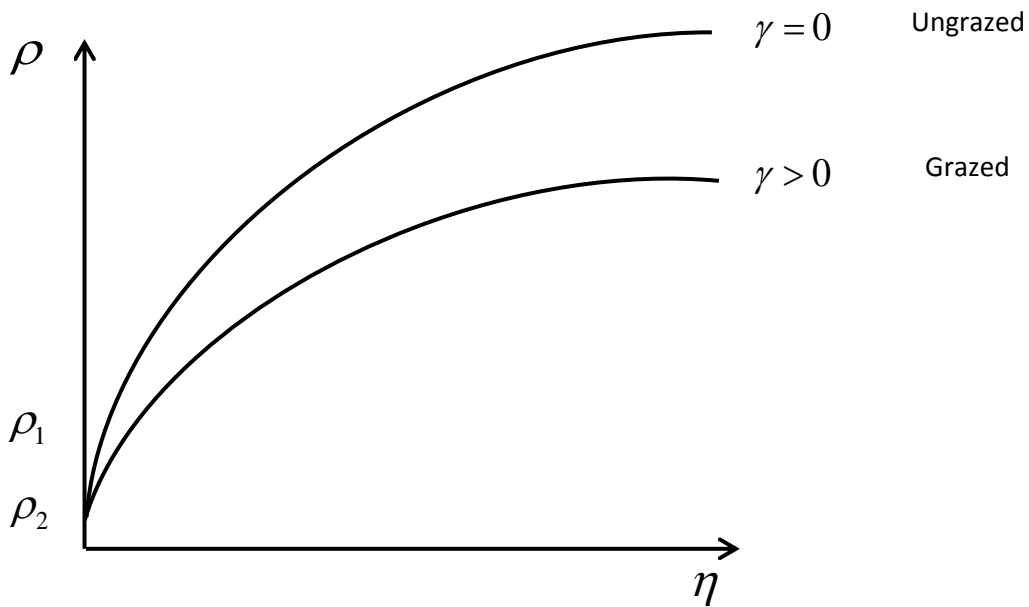
Figure 3: Effects of Stocking Rate on Forage Growth and their Relationship with Soil Organic Matter.
